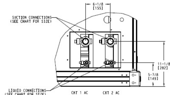
DETAIL A (NOTE POSITION OF CKT 1)
