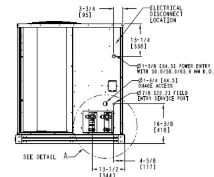
LEFT SIDE VIEW FOR 38AUD SYSTEMS
