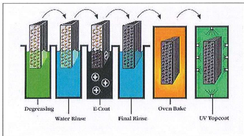
Fig 1 E-Coat Process
